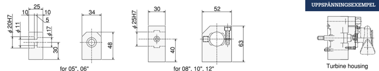
Turbine housing
