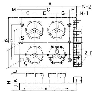
4-chucks montering
