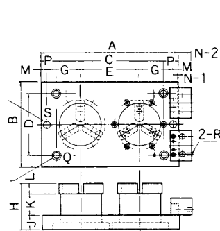
2-chucks montering
